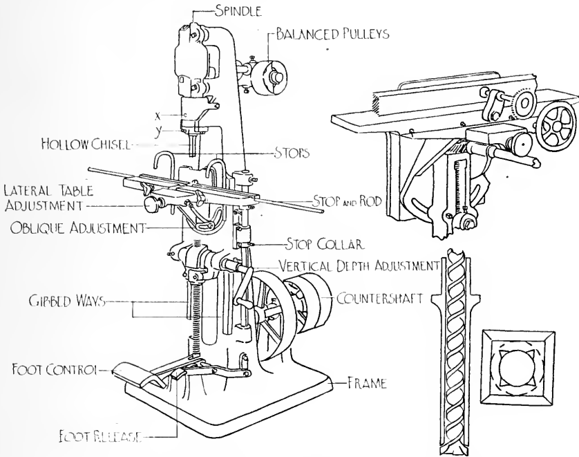
FIG. 194. VERTICAL HOLLOW CHISEL MORTISER.
